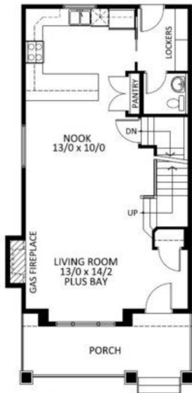
MAIN FLOOR PLAN 750 SQ.FT.
