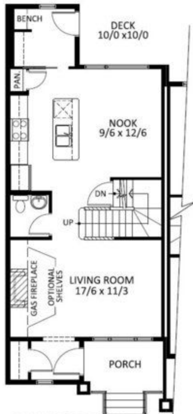
MAIN FLOOR PLAN 697 SQ.FT.
