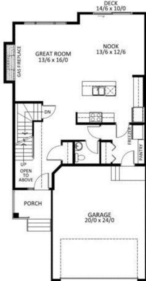
MAIN FLOOR PLAN 916 SQ.FT.
