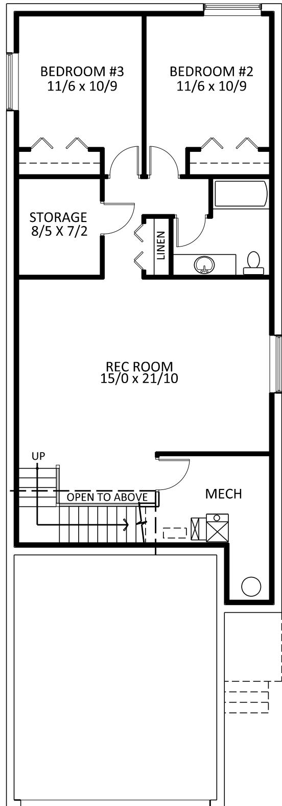
BASEMENT DEVELOPMENT 928 SQ.FT.
