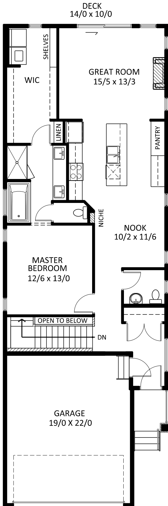
MAIN FLOOR PLAN 1171 SQ.FT.
